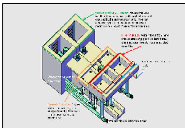
Stacked Rapid Sand Filter
