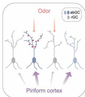
Fig. 8. Model schematic. Schematic of the proposed mechanisms for the context-dependent, cell-type specific plasticity. Coincidence of odor input and context-dependent piriform feedback input leads to increased apical spine density (red) and stronger and faster responses (shown by darker color) of abGCs.
