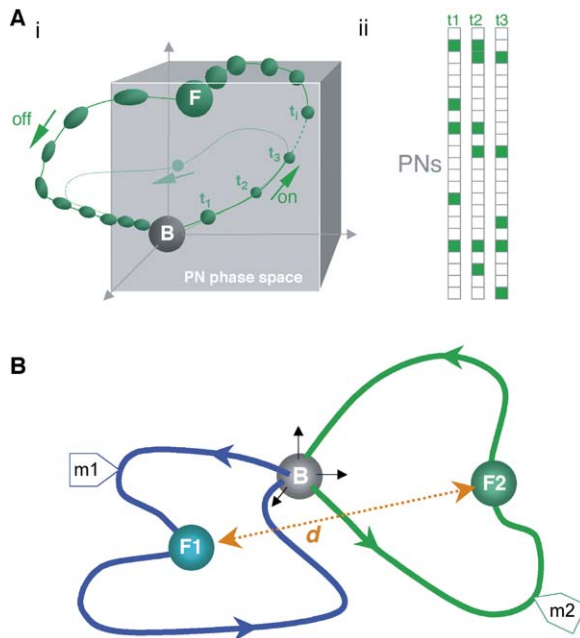
Figure 8. Schematic Diagram of Odor-Evoked PN Activity (A i) Idealized odor trajectory in PN space. B , baseline; F , fixed point; t_i , times corresponding to one oscillation cycle. During the on transient, synchronization is the highest and most spikes occur within a single 10–20 ms period. Activity thus “hops” from one oscillation cycle to the next while the identities of the responding PNs evolve (see [A ii]). (A ii) Evolving PN activity that underlies the trajectory in (A i), green squares represent responsive PNs. (B) Idealized trajectories for two different odors. Odor trajectories differ at their fixed points ( F1 and F2 ) but are maximally distant during the transient response phases (e.g., m1 and m2 ). ( d , Euclidian distance.)
