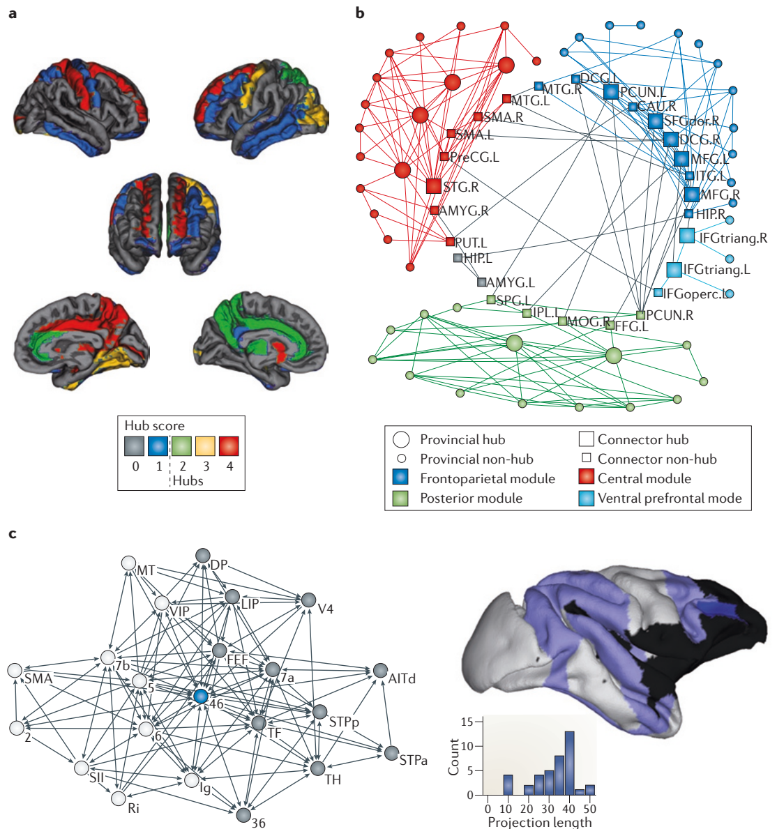
Figure 2 | Hubs and modules in the brain. a | In human brain networks, some regions have more connections to the rest of the network, greater clustering, shorter path-lengths and greater betweenness centrality (that is, they mediate a greater proportion of the shortest path connections between other regions). Such regions are called 'hubs' and include parts of medial parietal cortex, cingulate cortex and superior frontal cortex, indicated here by their 'hub score' (regions with a hub score of 2 or higher are defined as hubs). The hub score is based on the ranking of the brain region relative to other regions in terms of numbers of connections, centrality, clustering and path length 139 . b | Human brain networks are also modular. Brain regions are colour-coded according to their membership in major modules comprising frontal (dark blue), central (red) and posterior (green) brain regions as well as a smaller module of inferior frontal regions (light blue). The connector hubs, which mediate most of the longer-distance inter-modular connections, are shown as a ring of square markers 107 . c | Connector hubs are often regions of multimodal association cortex. For example, Brodmann area 46 (blue circle in left panel; dark blue area in right panel) in the dorsolateral prefrontal cortex of the macaque brain has a large number of long-distance connections (inset) to remote brain areas 73 . The figure shows area 46 as a hub connecting two modules (indicated in white and grey). Part a is reproduced, with permission, from REF. 139 © (2010) Society for Neuroscience. Part b is reproduced, with permission, from REF. 107 © (2010) Frontiers Media. Part c is reproduced from REF. 73. AITd, anterior inferotemporal (dorsal); AMYG, amygdala; CAU, caudate; DCG, middle cingulate and paracingulate gyri; DP, dorsal parietal; FEF, frontal eye fields; FFG, fusiform gyrus; HIP, hippocampus; IFGoperc, inferior frontal gyrus, opercular part; IFGtriang, inferior frontal gyrus, triangular part; Ig, insular cortex (granular); IPL, inferior parietal lobule; ITG, inferior temporal gyrus; LIP, lateral inferior parietal; MFG, middle frontal gyrus; MOG, middle occipital gyrus; MTG, middle temporal gyrus; PCUN, precuneus; PreCG, precentral gyrus; PUT, putamen; Ri, retroinsular cortex; SFCdor, superior frontal cortex, dorsal part; SII, secondary somatosensory area; SMA, supplementary motor area; SPG, superior parietal gyrus; STG, superior temporal gyrus; STPa, superior temporal polysensory (anterior); STPp, superior temporal polysensory (posterior); VIP, ventral inferior parietal; .L, left; .R, right.
