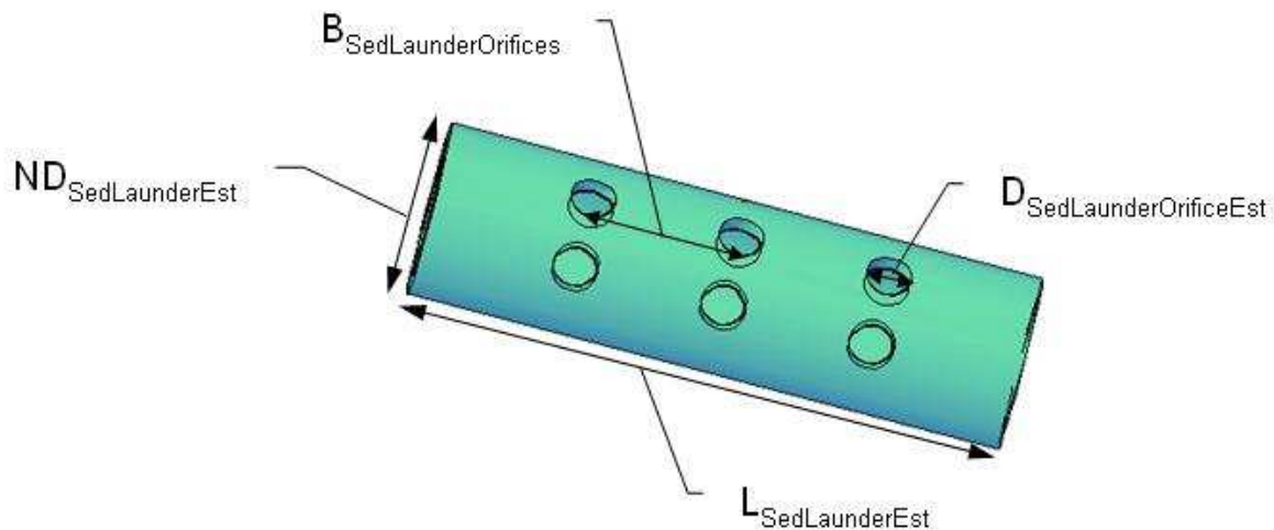
Figure 12: Effluent Launder Design
