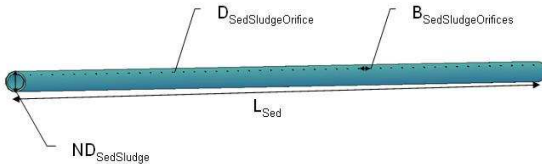
Figure 10: Sludge Drain
