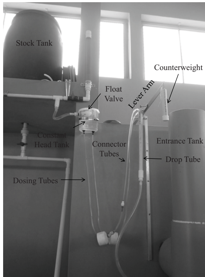
Figure 2.8: LCDC in operation at the Alauca municipal water treatment plant in Alauca, Honduras. Plant flow rate is 12 L/s .
