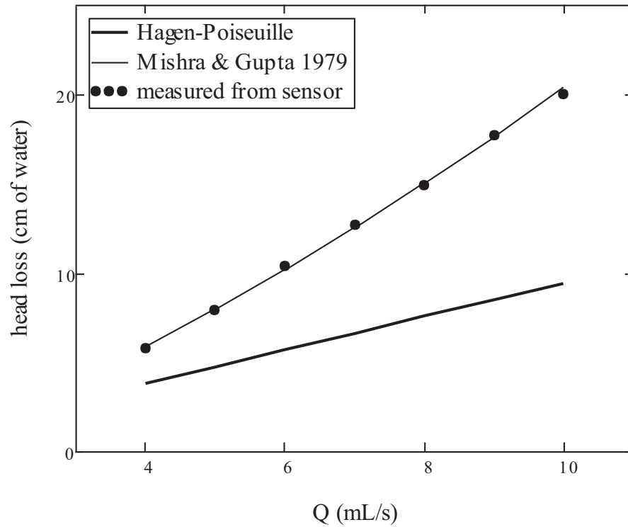
Figure 3.4: Comparing head loss across a 18.64 m tube flocculator measured by a pressure sensor and values computed using the Mishra and Gupta (1979) correlation factor. Hagen-Poiseuille prediction for straight pipe flow is shown for comparison.
