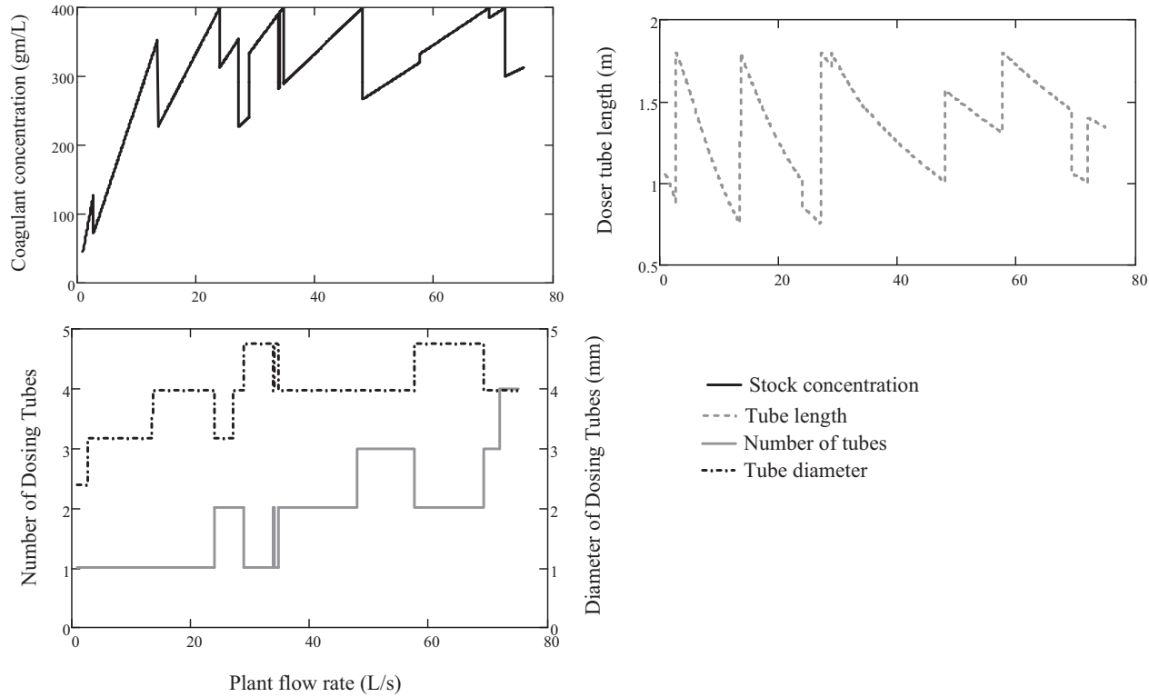
Figure 2.4: LCDDC design algorithm results for plant flow rates 1 – 75 L/s. As the flow rate changes, the dominating constraint may change causing the values given by the algorithm to fluctuate. The discontinuities shown are caused by the discrete sizes of tubing and the requirement of an integer number of tubes. For example at approximately 3 L/s the algorithm changes the specified diameter of the dosing tube from 2.38 mm ( 3/32 in) to 3.175 mm ( 1/8 in) and the doser tube length and coagulant concentrations must both change to maintain constant dose.
