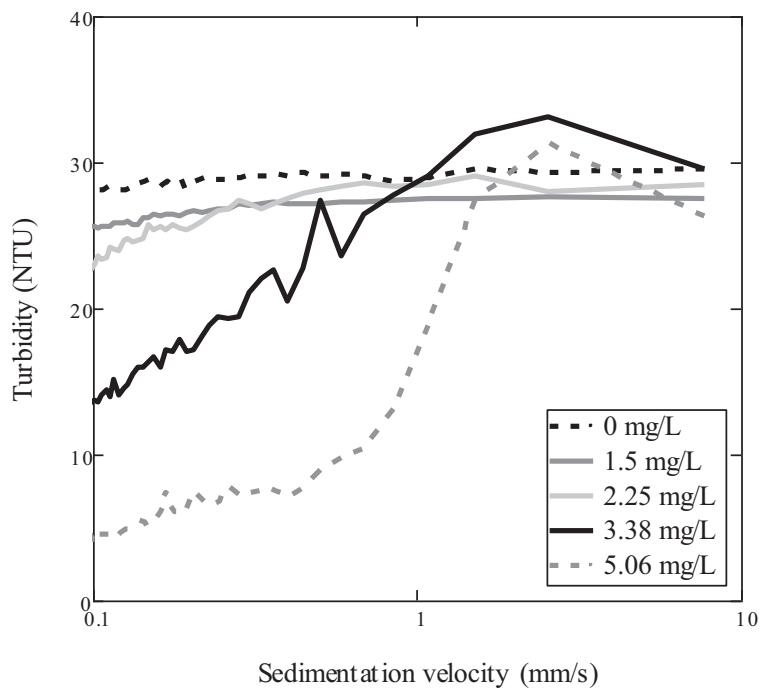
Figure 3.10: Smoothed data sets with varying alum doses.
