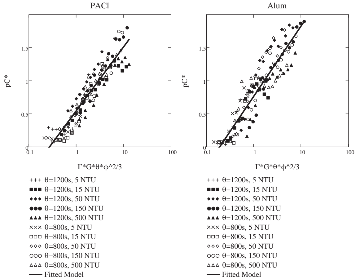
Figure 5.6: Model fit for pC^* as a function of effective collision potential for V_{Capture} = 0.12 \frac{mm}{s} . Sample size, N , is 136 for PACI and 140 for Alum. R_{PACI}^2 = 0.92 and R_{Alum}^2 = 0.89 .
