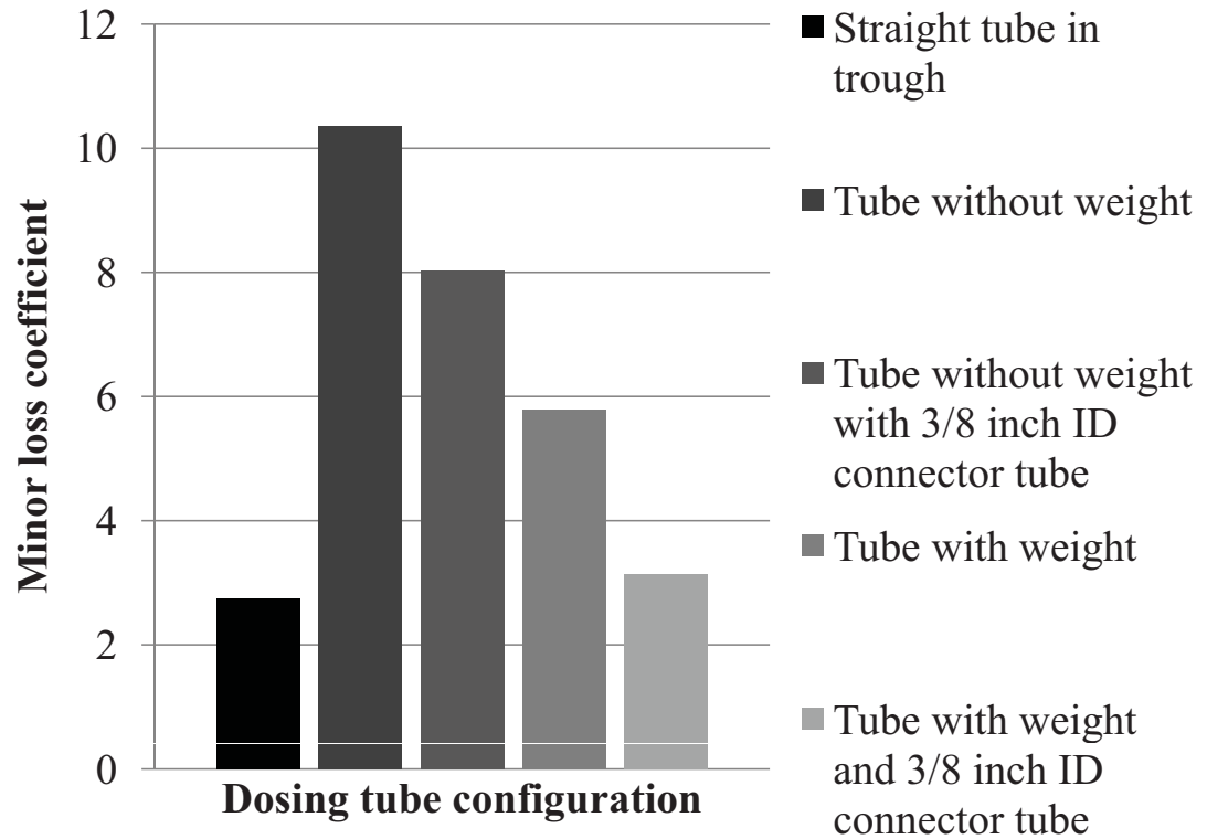
Figure 2.5: Minor loss coefficients for alternative tubing configurations. Values are an average of three trials for a 1.42 m dosing tube over a range of head losses (0. – 20 cm).
