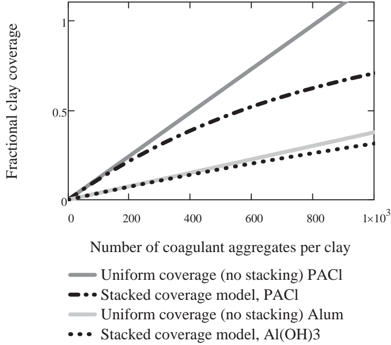
Figure 5.3: Fractional clay surface coverage for PACl and Al(OH)_3 .
