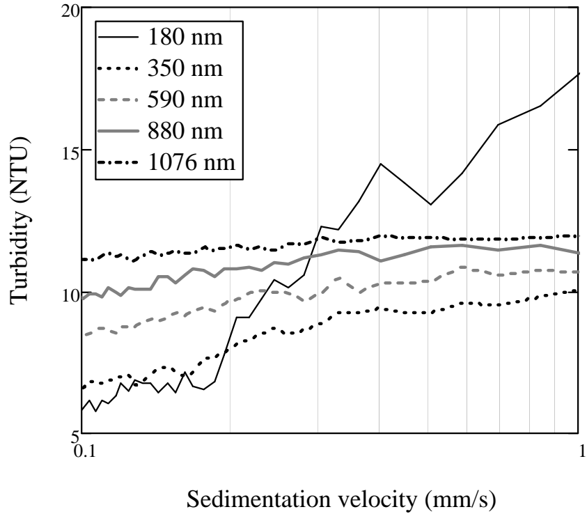
Figure 4.8: Sedimentation velocity from PACl aggregates of various sizes. The vertical line represents the capture velocity, the sedimentation velocity at which the residual turbidity measurement is taken. Data was collected at 1 second intervals for 30 minutes of settling. Each plot consists of 50 data points, each an average of 36 seconds of data.
