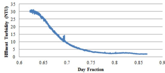
Figure 5: Effluent turbidity as a function of time with 5 mg/L of humic acid and 0.5 mg/L of coagulant. Day fraction corresponds to the fraction in a 24 hour period.
