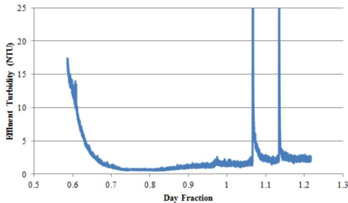
Figure 8: Effluent turbidity as a function of time with 5 mg/L of humic acid and 1.5 mg/L of coagulant. This set of experiment yielded a lowest effluent turbidity value of 0.56 NTU.
