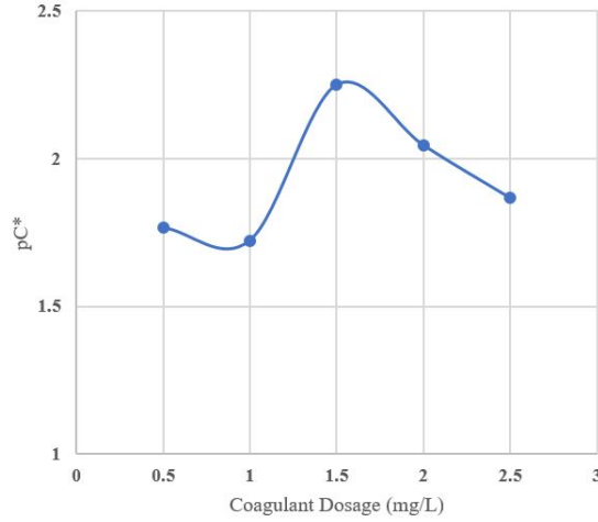
Figure 13: Turbidity removal efficiency as a function of coagulant dosage at 5 mg/L humic acid concentration.
