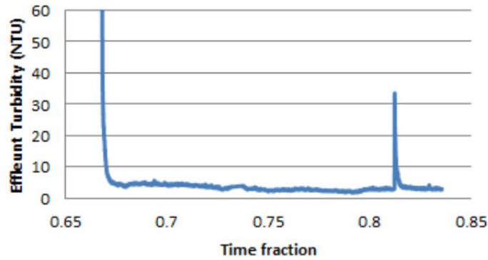
Figure 7: Effluent turbidity as a function of time with 5 mg/L of humic acid and 1.0 mg/L of coagulant. Day fraction corresponds to the fraction in a 24 hour period.
