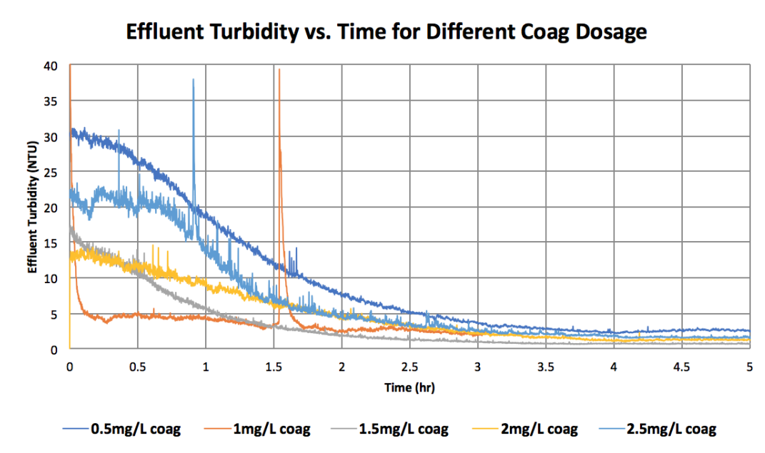
Figure 11: Effluent turbidity change vs time for different coagulant dosages ranging from 0.5mg/L to 2.5mg/L at 5mg/L HA
