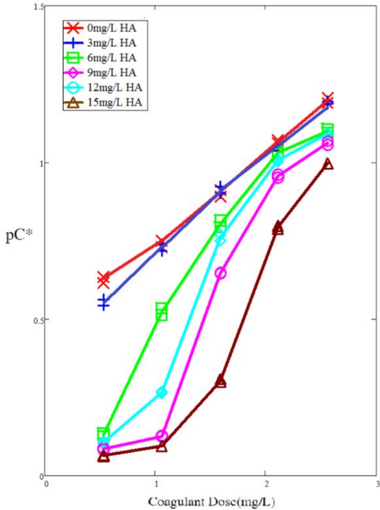
Figure 1: Yingda’s plot of turbidity at 50 NTU versus the coagulant dosage for various HA concentration.
