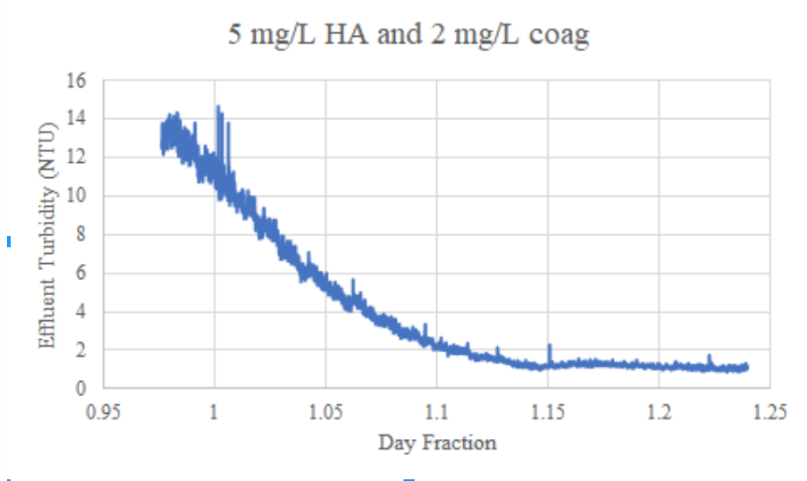
Figure 9: Effluent turbidity as a function of time with 5 mg/L of humic acid and 2.0 mg/L of coagulant. This set of experiment yielded a lowest effluent turbidity value of 0.9 NTU.
