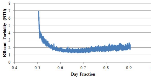
Figure 14: Effluent turbidity as a function of time at 10 mg/L of humic acid and 2 mg/L of coagulant.
