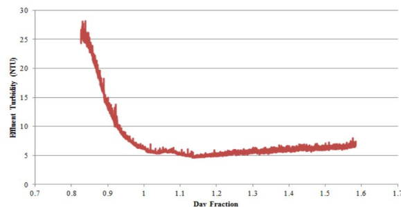
Figure 6: Effluent turbidity as a function of time with 5 mg/L of humic acid and 1.0 mg/L of coagulant. Day fraction corresponds to the fraction in a 24 hour period.
