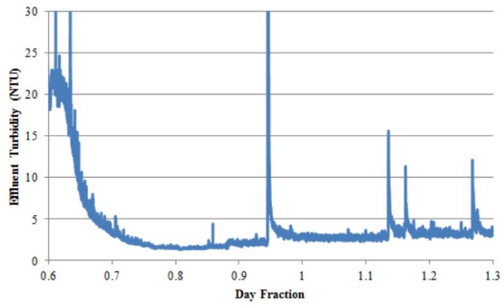
Figure 10: Effluent turbidity as a function of time with 5 mg/L of humic acid and 2.5 mg/L of coagulant. This set of experiment yielded a lowest effluent turbidity value of 1.36 NTU.
