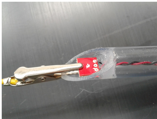
Figure 15: A small clip was used as a clamp to hold the photosensor in place while the clear, waterproof silicone dried. This picture was taken before an additional layer of silicone was used to cover and thus waterproof the top and bottom of the photosensor. A gap was left between the first and second layers so that the silicone would not block light from the phototransistor.
