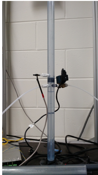
Figure 16: Initial setup of original gas sensor
