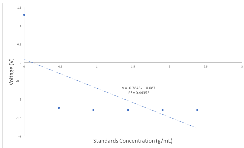
Figure 15: The relationship between output voltage (V) and the solids concentration of granules (g/mL). At concentrations above 0 g/mL, the output voltage was similar to the measured dark voltage, indicating that light was not able to pass through the experimental tube.
