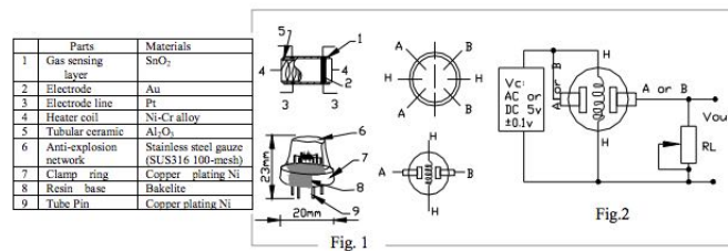
Figure 1: Design of the MQ-4 methane sensor made by Henan Hanwei Electronics Company, Ltd. (Henan Hanwei Electronics Co., Ltd., 2016)
