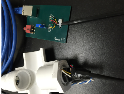
Figure 12: The LED and ambient light sensor are on opposite sides of the four-way pipe and ultimately are connected to respective positions on the breadboard. The breadboard can be connected to the ProCoDa box through the thick blue wire connector.
