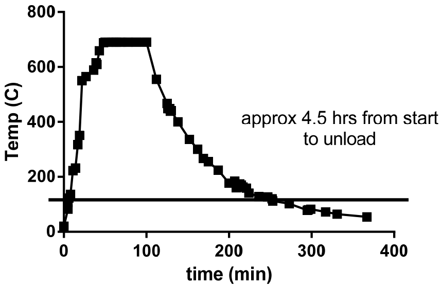
Pyrolysis furnace
