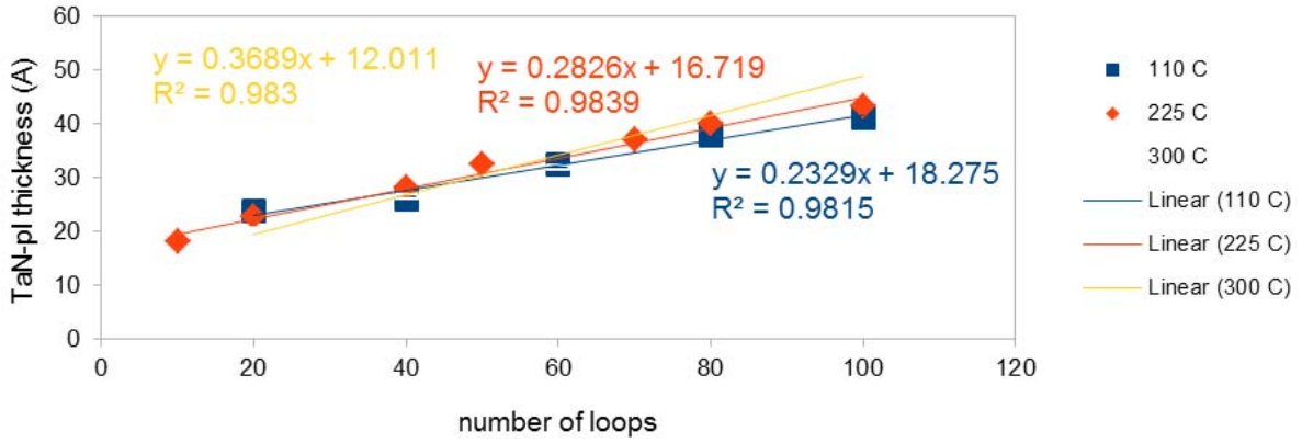
TaN-pl index of refraction v. thickness
