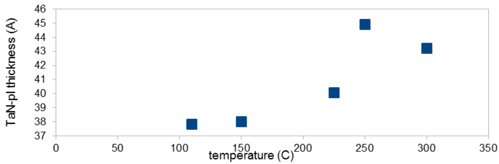
TaN-pl thickness v. temperature
