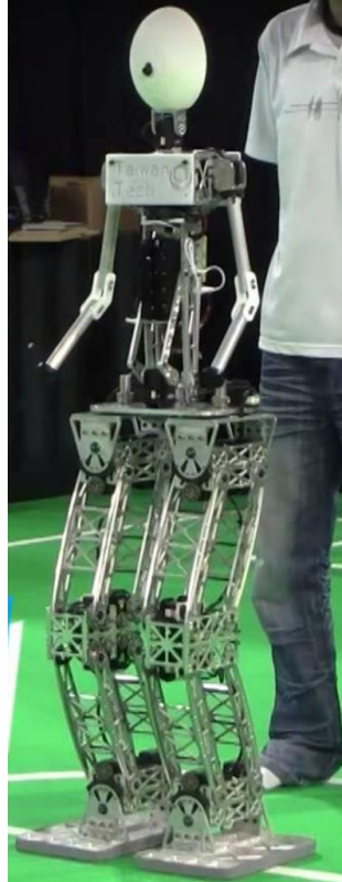
Figure 4: 2013 RoboCup Adult Size Humanoid League Runner-up: Team Taiwan
