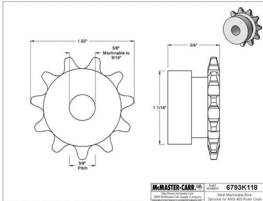
Figure 28: Sprocket Drawing
