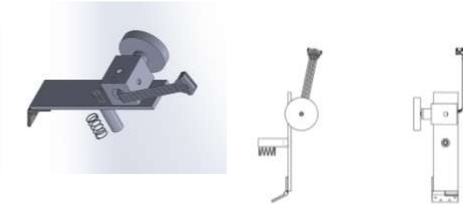
Figure 4: Head Motor Mount detailed CAD and detailed schematic
