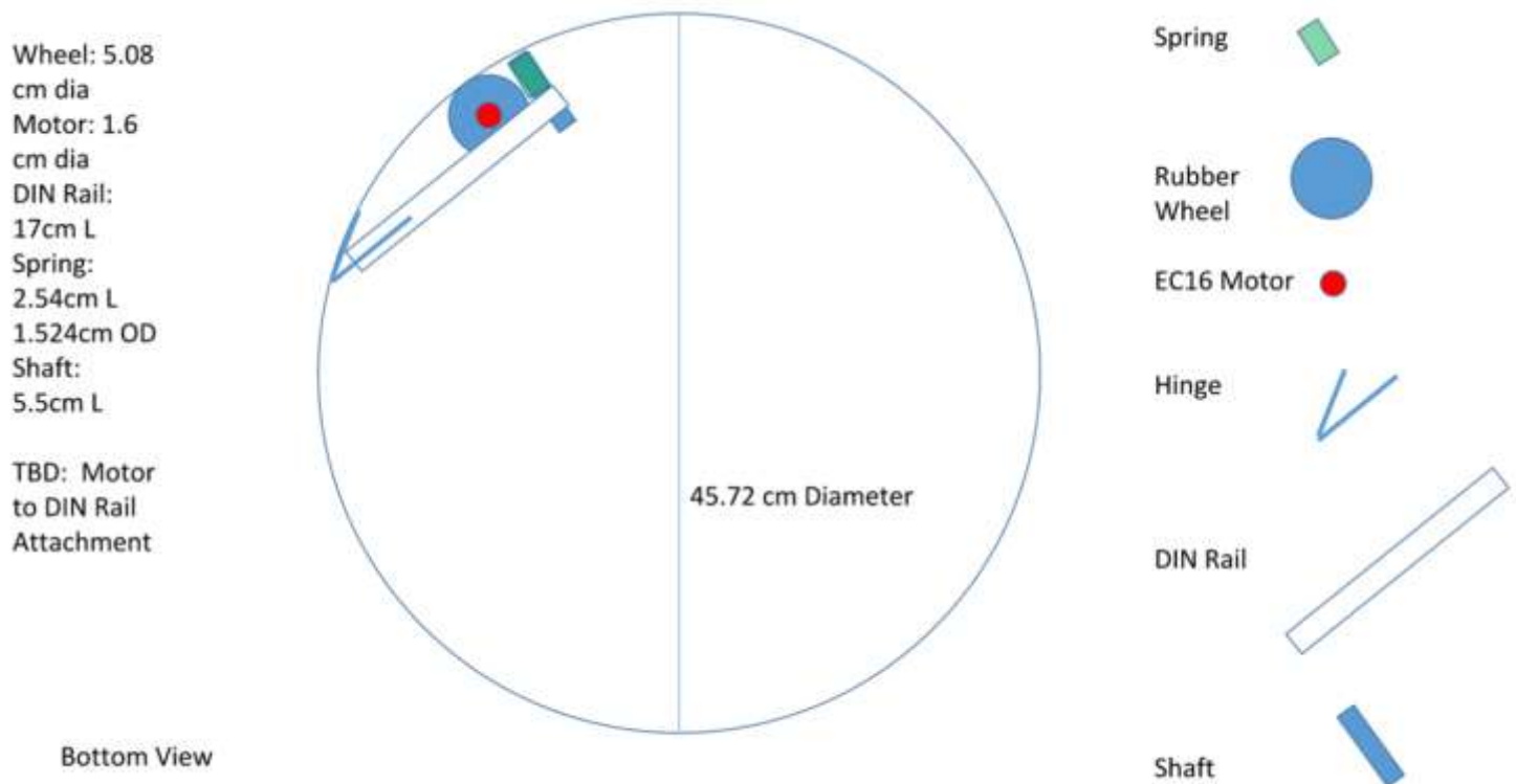
Figure 3: Motor mounting schematic
