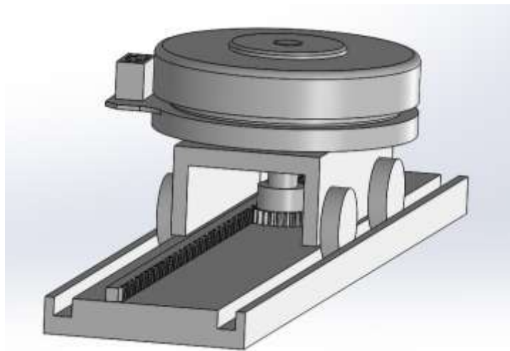
Figure 59: CAD for iterated mechanism with motor
