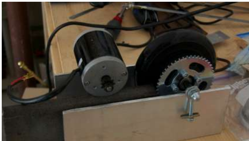
Figure 11: Researched locomotion design #1
