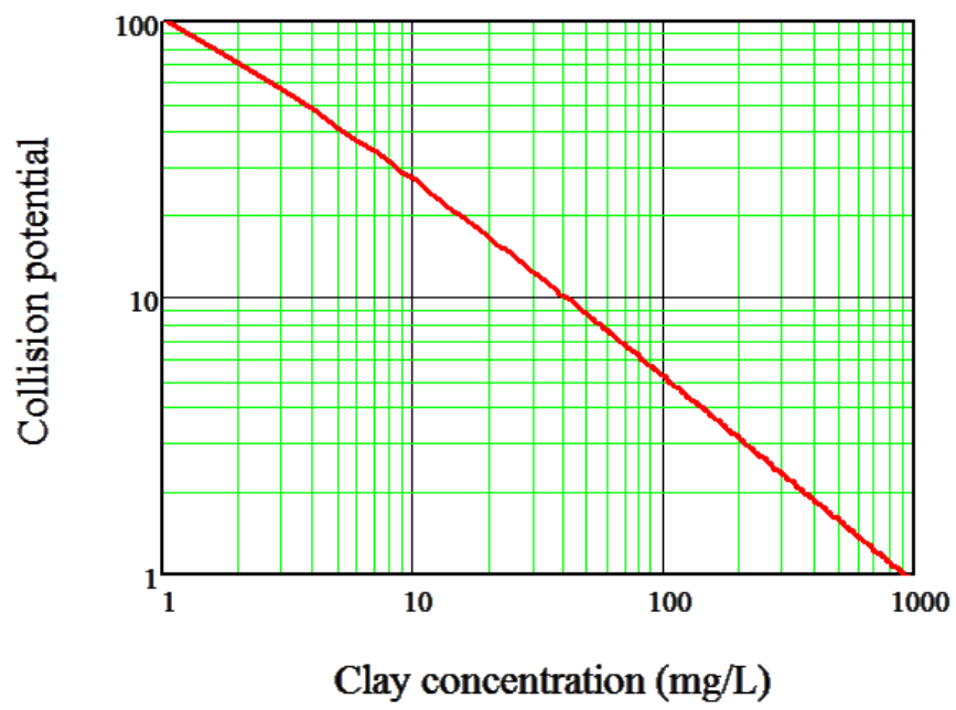
Figure 1: Required collision potential m^{\frac{2}{3}} as a function of the clay concentration in the flocculator based on the fractal flocculation model.
