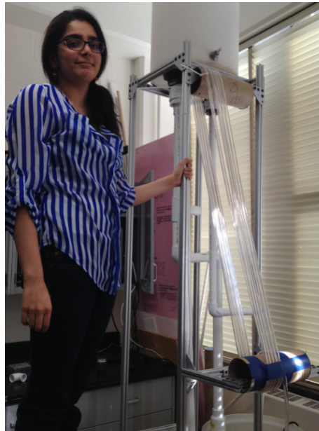
Figure 3: Team Member Ruju with the Head Loss System
