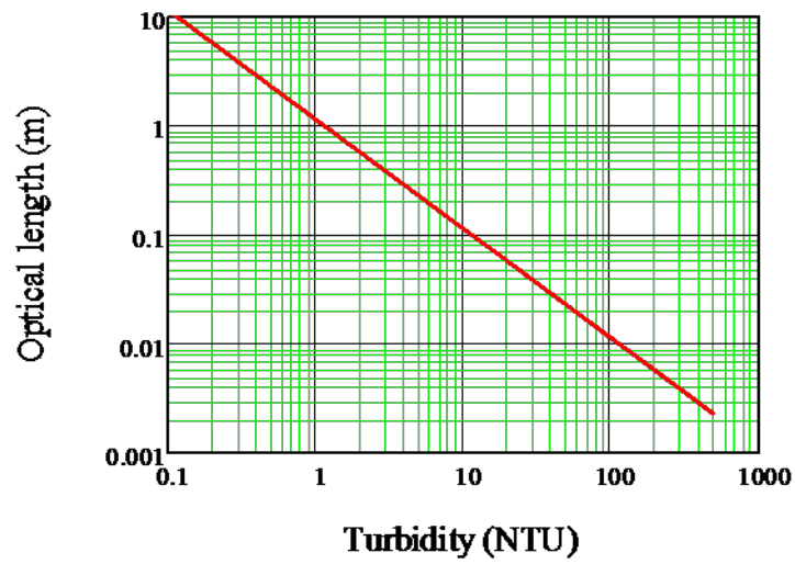
Figure 2: Optical depth vs turbidity based on the assumptions that the clay is 1 \mu\text{m} in diameter and that the display is obscured when an average of one clay particle blocks the light path.
