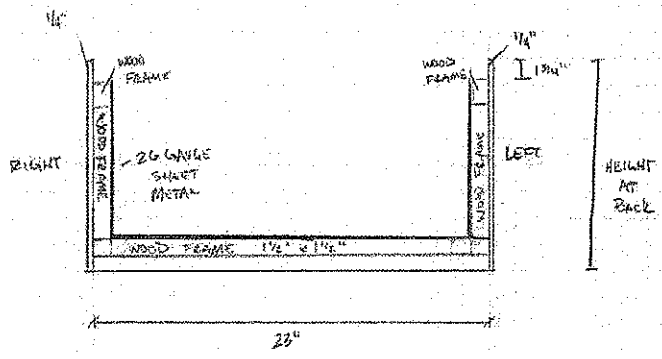
CROSS SECTION AT BACK OF BOX
