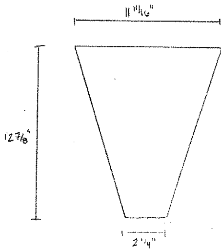
TRAPEZOID PANELS QNT 4
