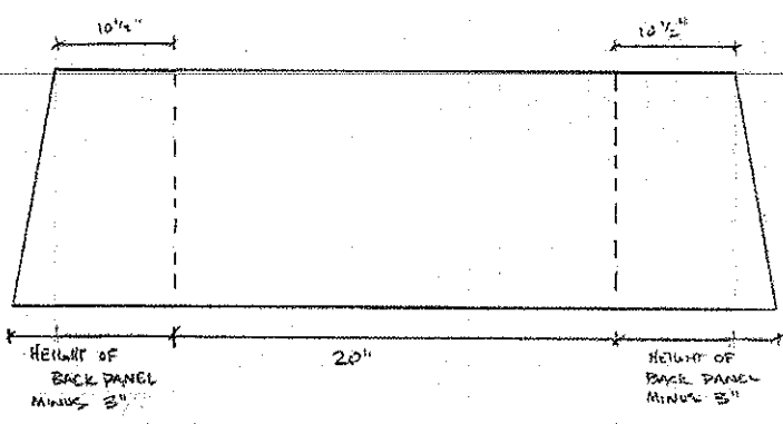
BOTTOM AND SIDE PANEL SHEET METAL
