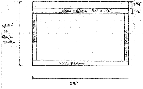
BACK PANEL
