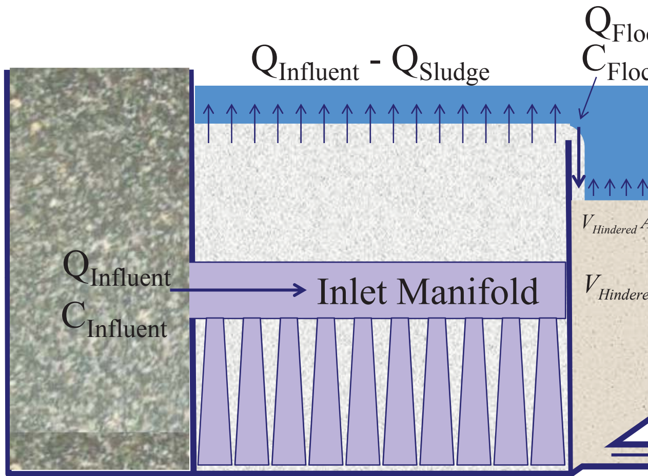
Figure 1: Mass balance for a flocculator, floc blanket, and floc hopper.
