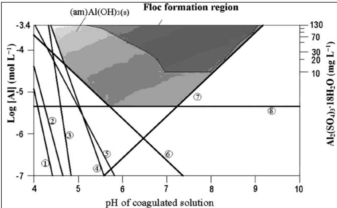
Figure 2-4. Aluminum solubility diagram in equilibrium with amorphous \text{Al(OH)}_{3(s)} based on thermodynamic data, and floc formation region based on experimental observations. Lines 1, 2, 3, 4, 5, 6, 7, 8 represent the concentrations of [\text{Al}_3(\text{OH})_4]^{5+} , [\text{Al}_2(\text{OH})_2]^{4+} , [\text{Al}_{13}\text{O}_4(\text{OH})_{24}]^{7+} , \text{Al}^{3+} , \text{Al(OH)}^{2+} , \text{Al(OH)}_2^+ , \text{Al(OH)}_4^- , \text{Al(OH)}_3(s) , respectively (Xiao et al., 2008b).
