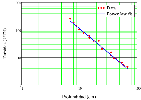
Figura 1: Turbidity can be measured based on depth of optical resolution.
