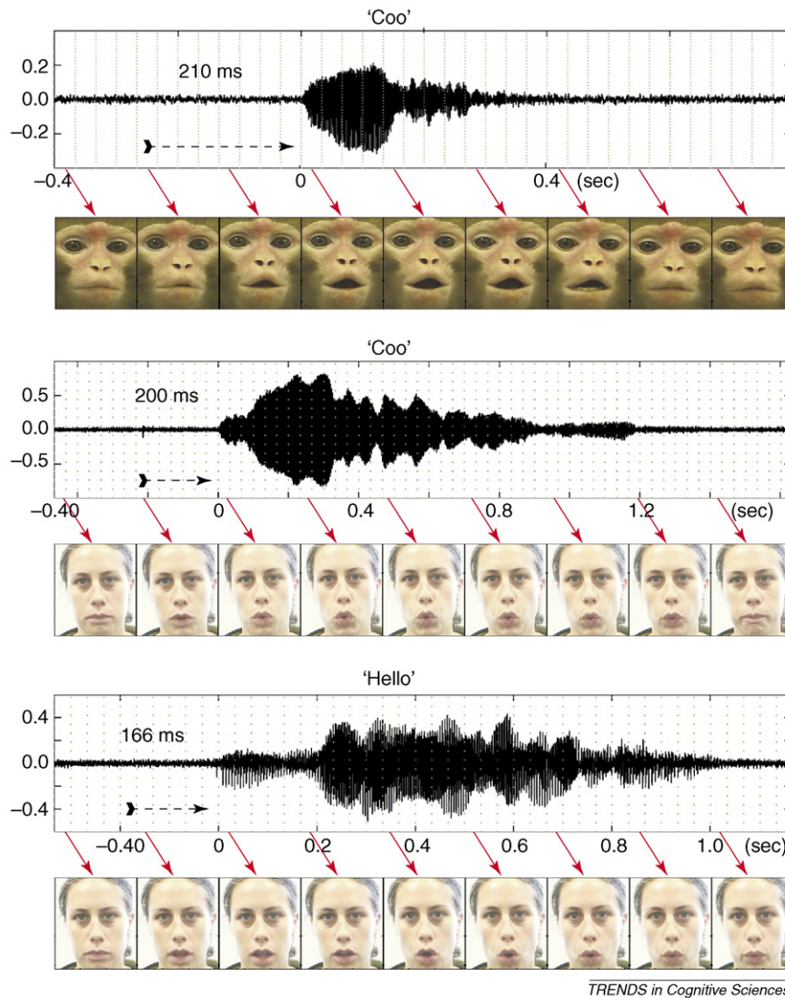
Figure 3. In order for visual inputs to modulate primary auditory processing, the ideal arrangement would be for visual inputs to arrive there before the time of auditory response onset. One factor that allows this to occur is the typical delay between visual articulatory gestures and the accompanying vocalizations. Examples of this visual-auditory offset are illustrated here, using a monkey making a 'coo' call (top), a human imitating this monkey coo (middle), and a human making a similar human vocalization ('hello', bottom). In each case, the auditory amplitude envelope of the call (sampled at 44.1 kHz) is displayed above a series of simultaneous video frames; these were acquired at 30 Hz (33.3 ms per frame), but only a key subset of the frames are shown, linked by arrows to the appropriate point in the auditory time line. The lag between the first detectable opening of the mouth and the onset of the auditory envelope function is displayed for each case (arrows and corresponding values in ms).
